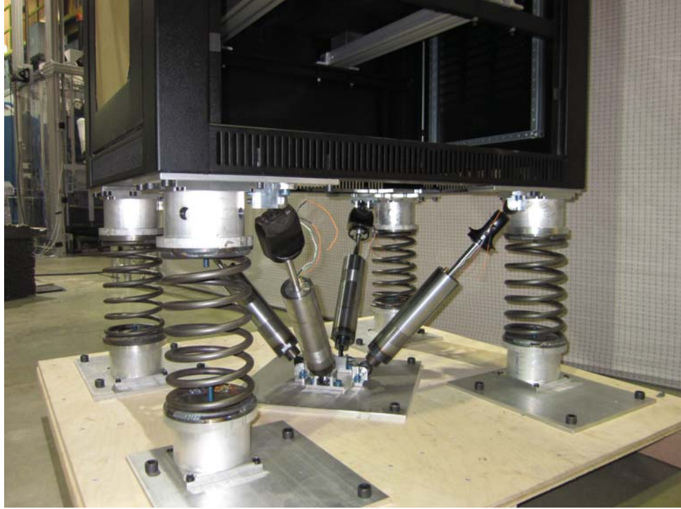
Figure 5.18: Pyramid configuration of suspension.
