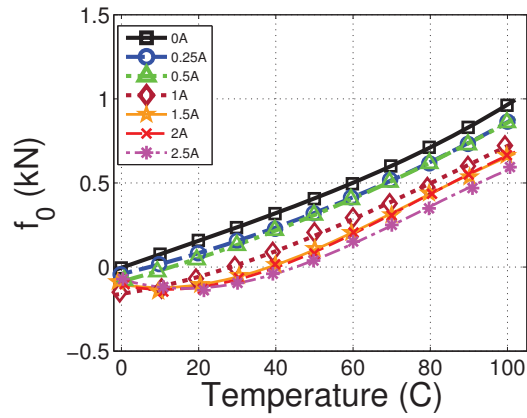
(a) Force offset f_0 .
