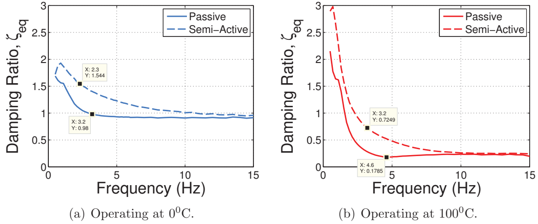
Figure 3.11: Equivalent damping ratio, \zeta_{eq} , as a function of excitation frequency with passive friction present in the system.
