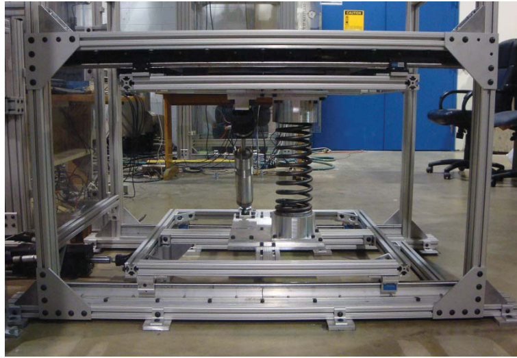
Figure 5.9: Lateral 1-DOF shake table test stand.
