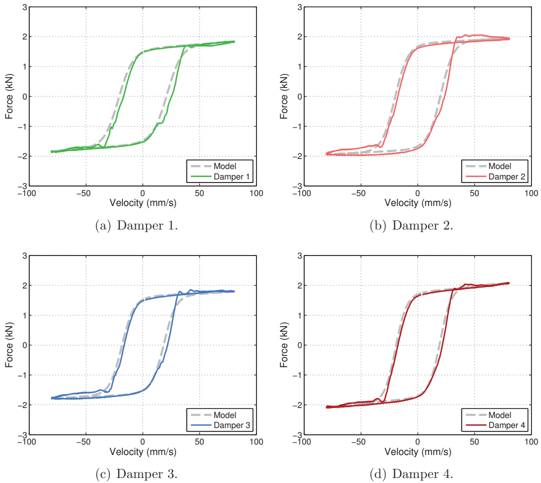
Figure 5.5: Measured and modeled force vs. piston velocity curves of the MR dampers at 2.5 A of applied current.
