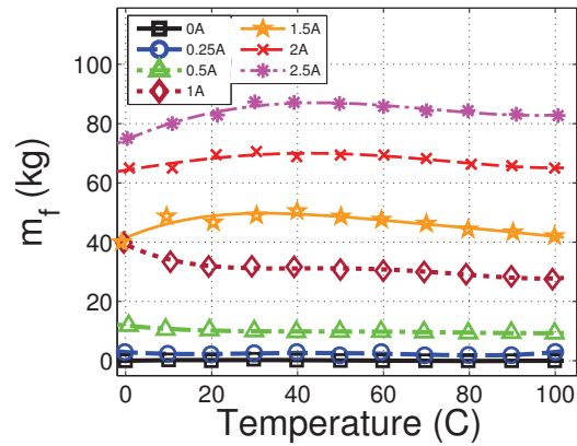
(c) Inertia m_f .
