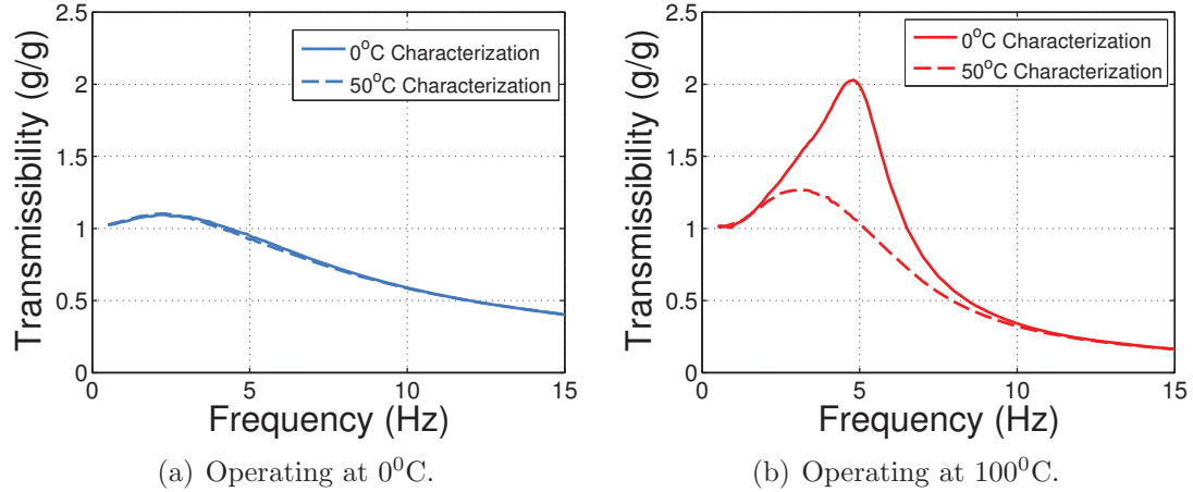
Figure 3.15: Frequency response for a 50 th percentile male when the MR damper is characterized at 0°C and 50°C, while the system is subjected to Skyhook control operating at two different temperatures.
