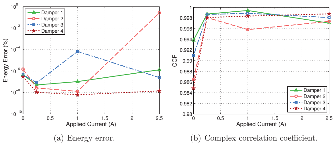
Figure 5.6: MR damper model correlation metrics.
