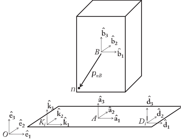
Figure 4.1: Coordinate frames of the 6-DOF system.
