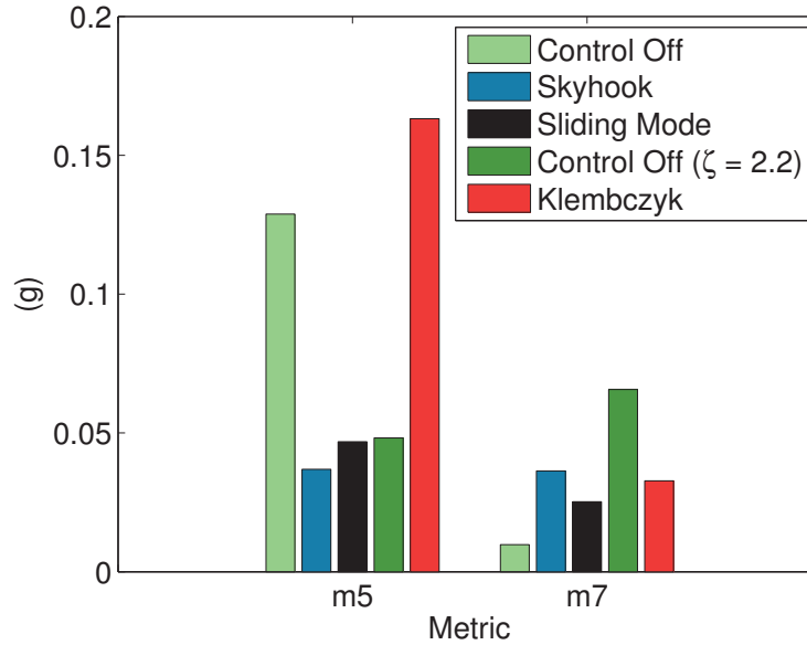
Figure 5.17: Performance metrics m_5 and m_7 from model.
