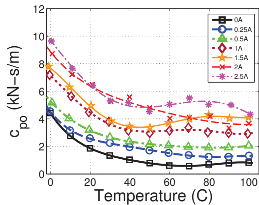
(e) Post-yield damping c_{po} .
