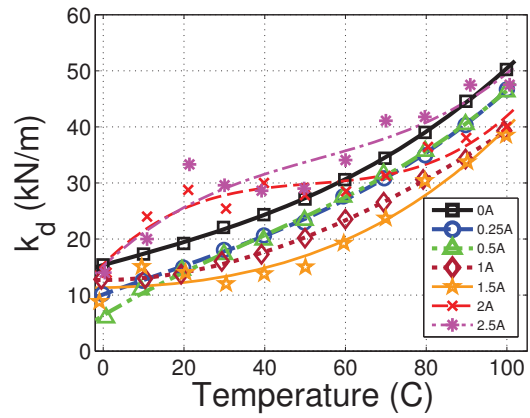
(b) Stiffness k_d .
