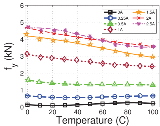
(f) Yield force f_y .
